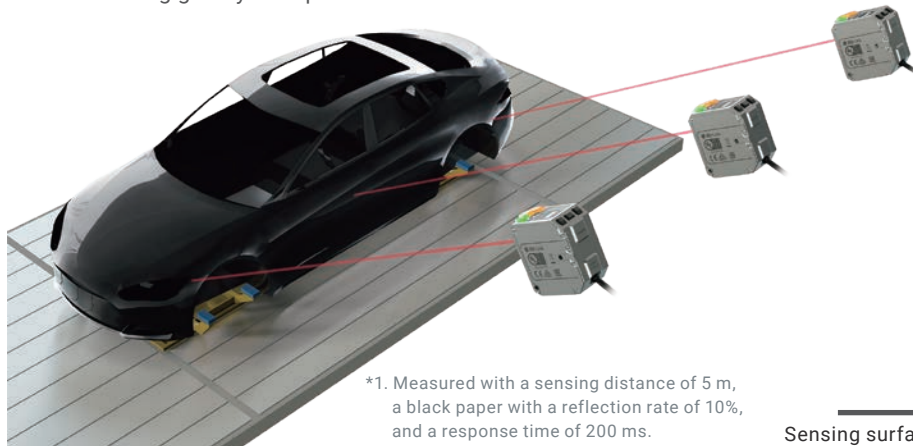
Detecting glossy black workpieces at a wide angle
